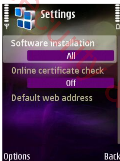
Software installation
