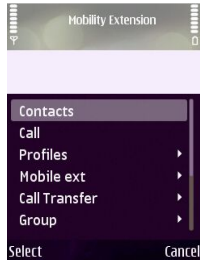
Main menu
