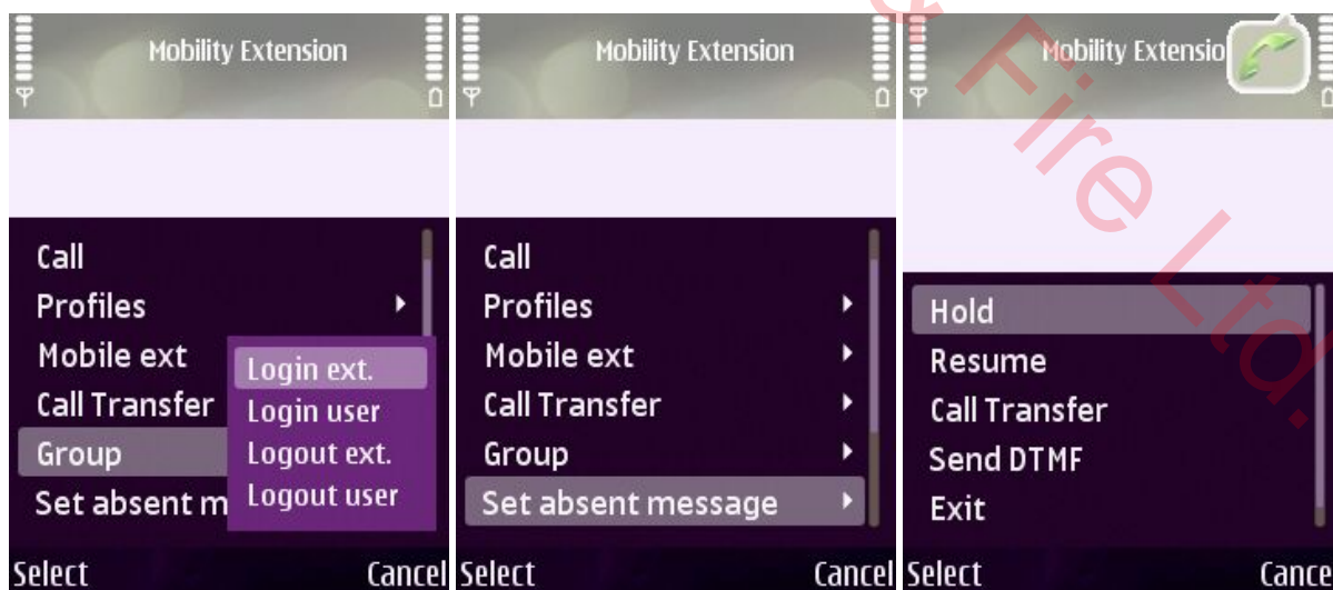
Logging in/out
